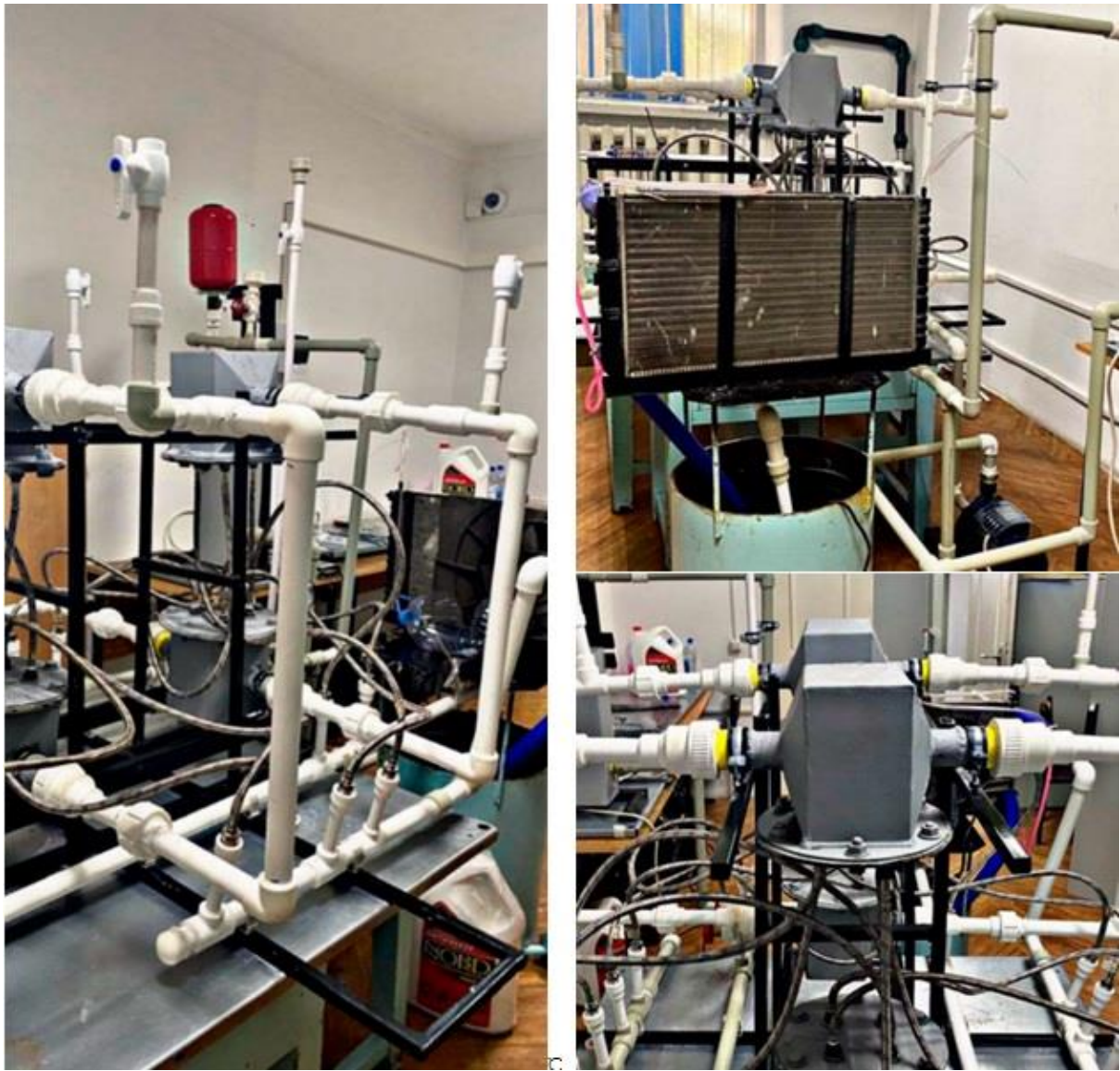
Figure 7. Experimental engine.
