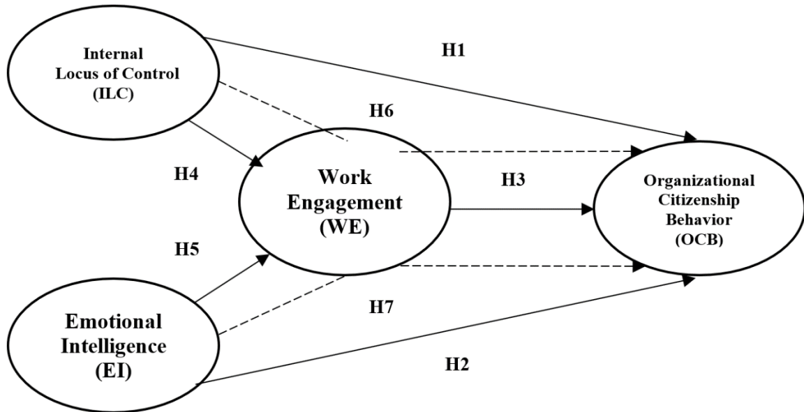
Figure 1. Research Framework.
